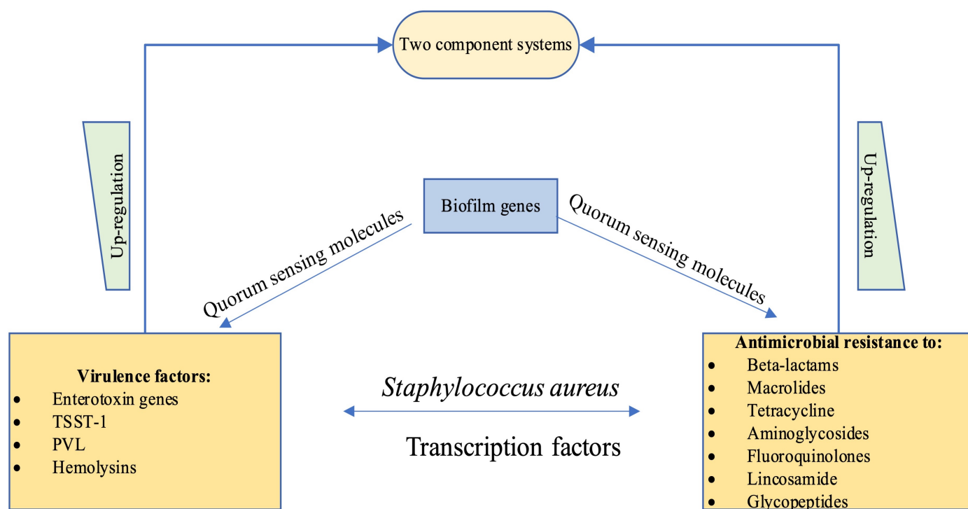
Fig. 3. Schematic representation of the interplay between antimicrobial-resistance genes and virulence determinants in Staphylococcus aureus (Patel and Rawat 2023)
