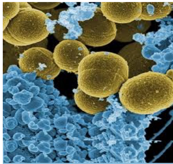
Fig. 1. Colonial morphology of Staphylococcus aureus on solid culture medium
