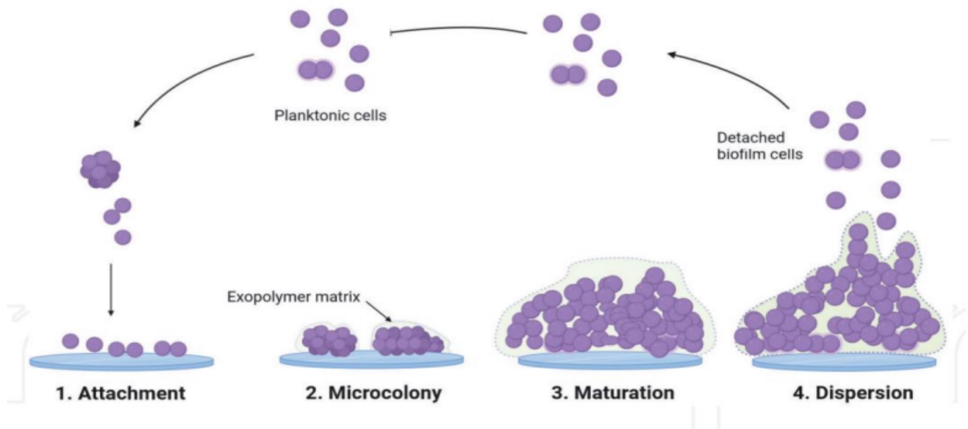
Fig. 2. Stages of biofilm formation by S. aureus (Alves Carneiro et al. 2020)
